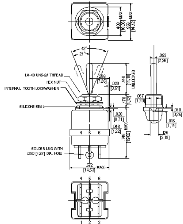
Terminal Identification
