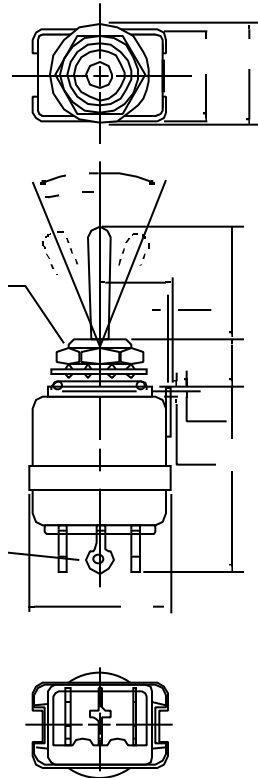
Terminal Identification
