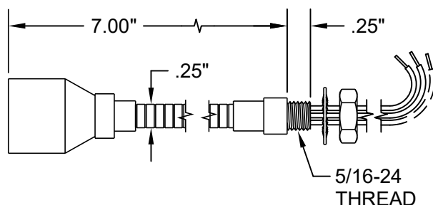
MAPLIGHT/OPLITE 4 - GOOSENECK
