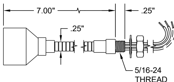
MAPLIGHT/OPLITE 6 - GOOSENECK
