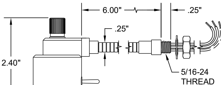
TASKLIGHT 600 - GOOSENECK
