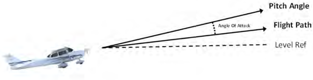
Figure 26: AoA Computation
