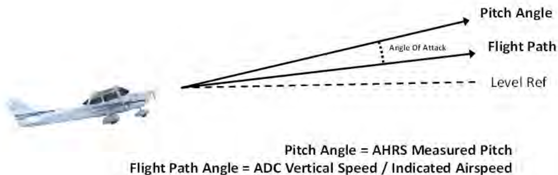
Figure 69: AoA Computation
