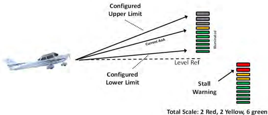
Figure 70: AoA Upper and Lower Limits
