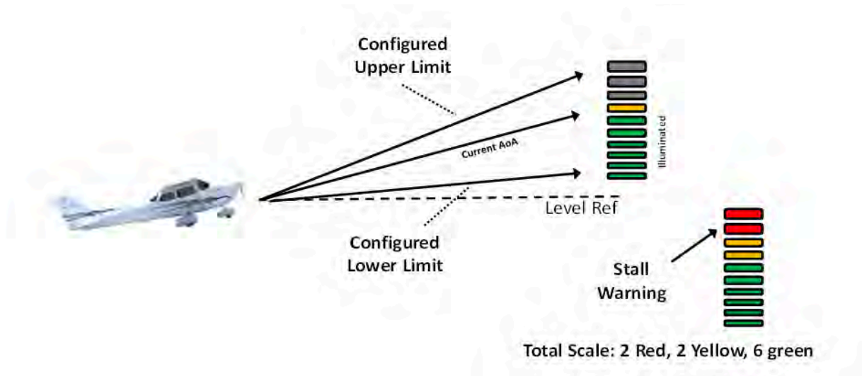
Figure 68: AoA Upper and Lower Limits
