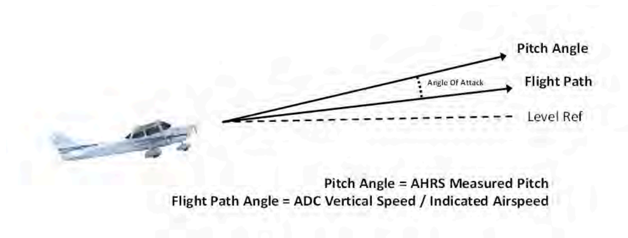
Figure 67: AoA Computation
