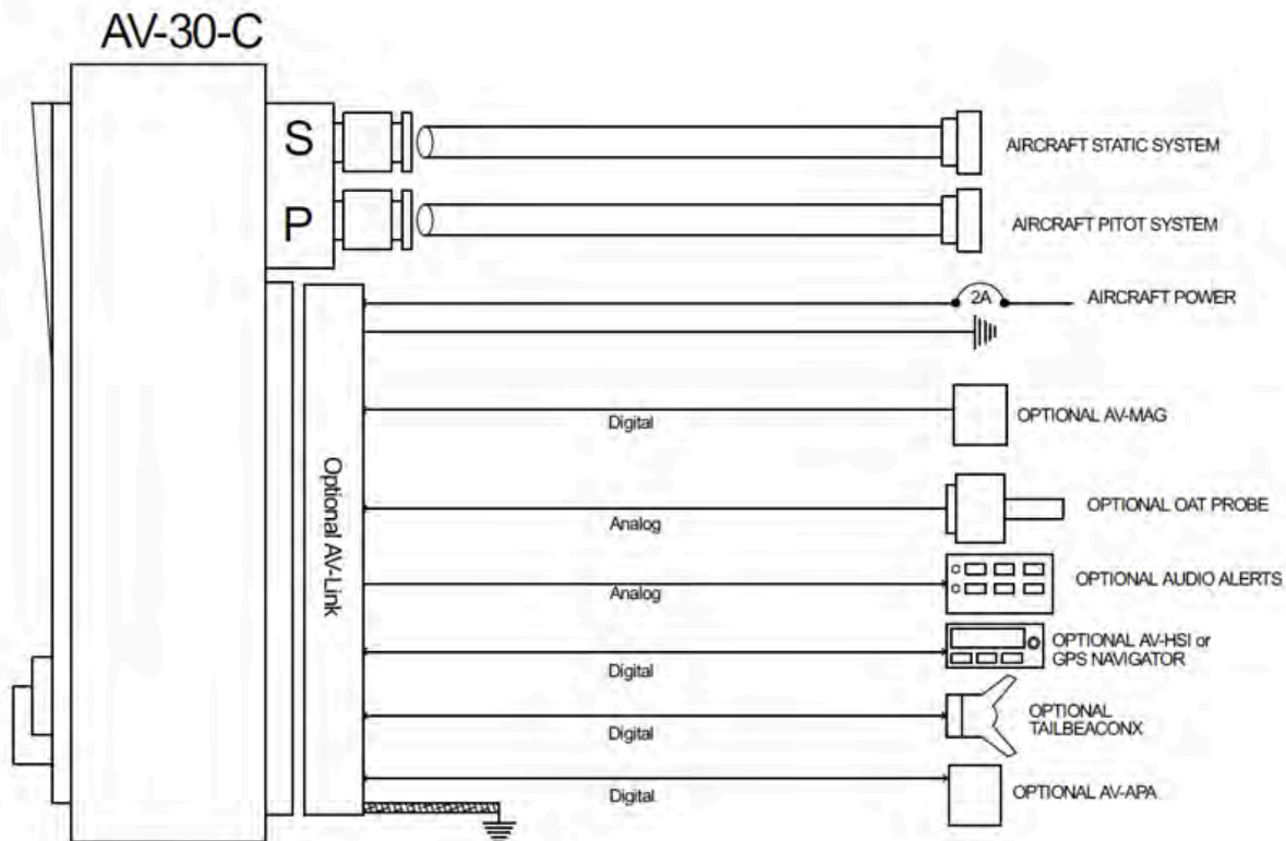
Figure 2: AV-30-C Aircraft Systems Interfaces – AI Mode
