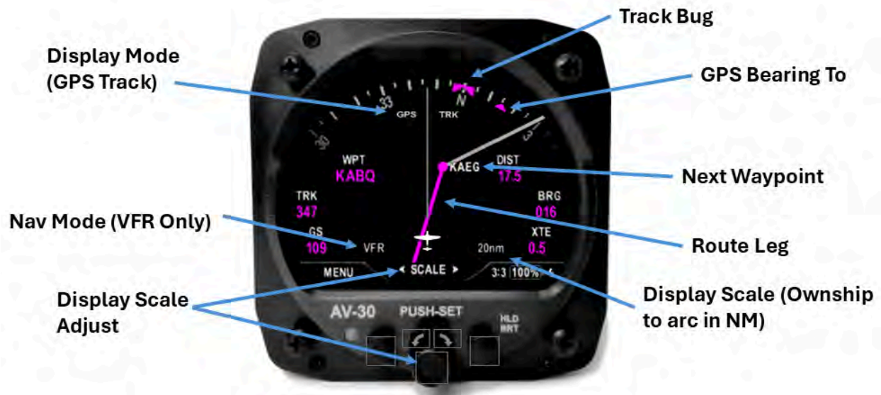
Figure 43: GPS Arc Mode
