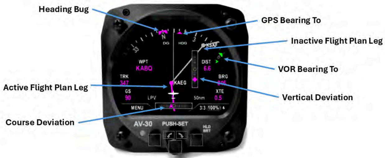
Figure 41: Arc Mode with Course Deviation and Glideslope
