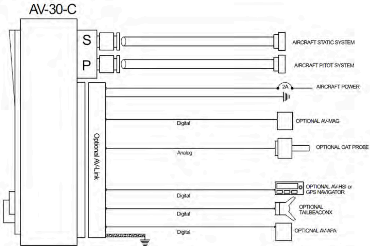
Figure 3: AV-30-C Aircraft Systems Interfaces – DG, MFD, or CDI Mode
