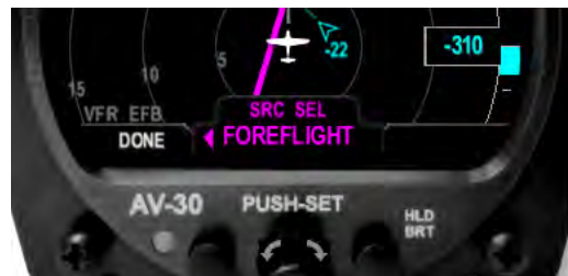
Figure 55: Wireless GPS on MFD
