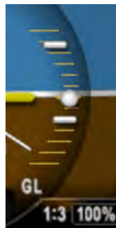
Figure 29: AI Mode, G-Load Indication
