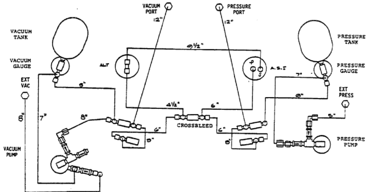
1811D PLUMBING SCHEMATIC DIAGRAM
