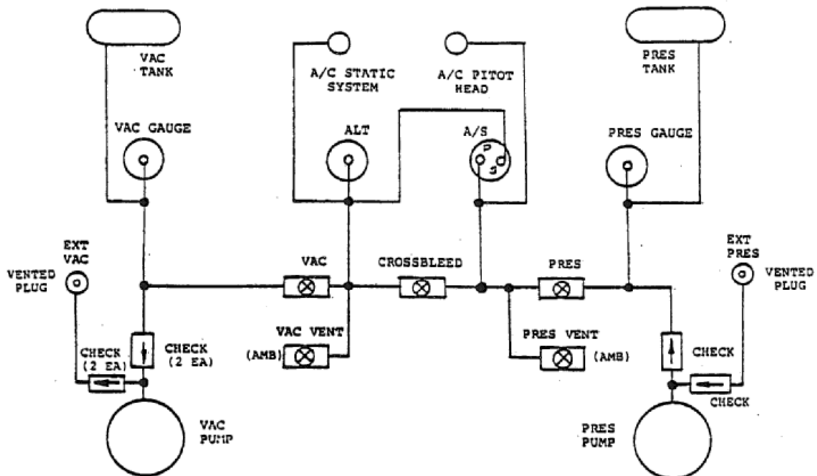
1811D OPERATIONAL SCHEMATIC DIAGRAM
